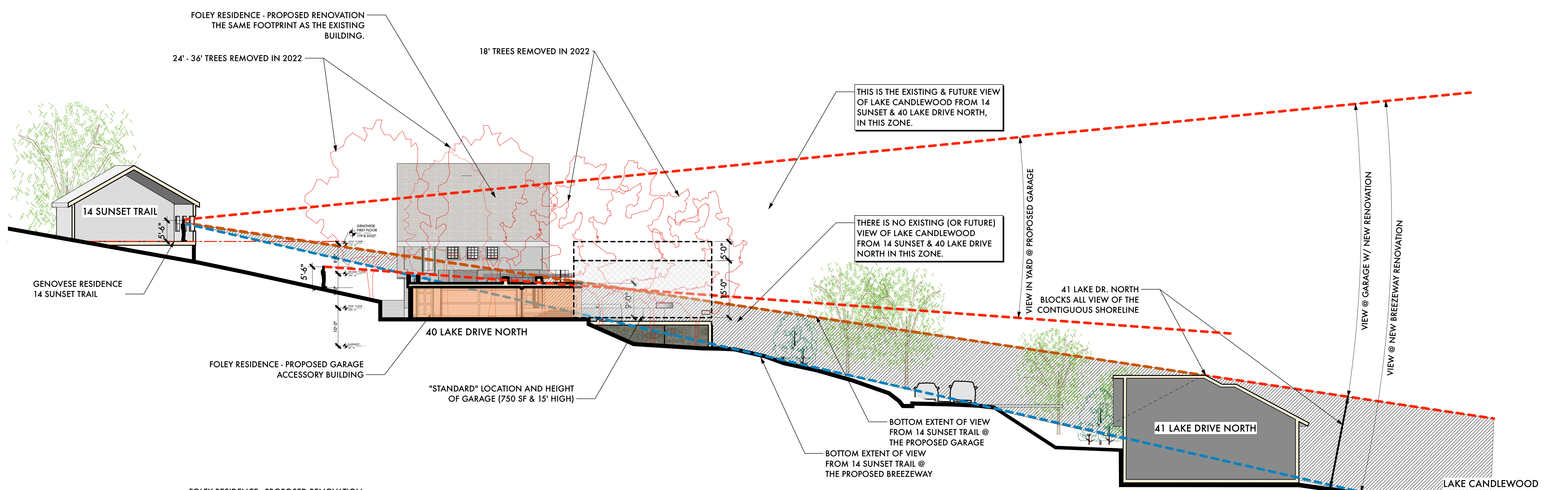
3 SITE SECTION A-A - VIEWS OF LAKE CANDLEWOOD @ PROPOSED GARAGE A-14 Scale: 1:150
