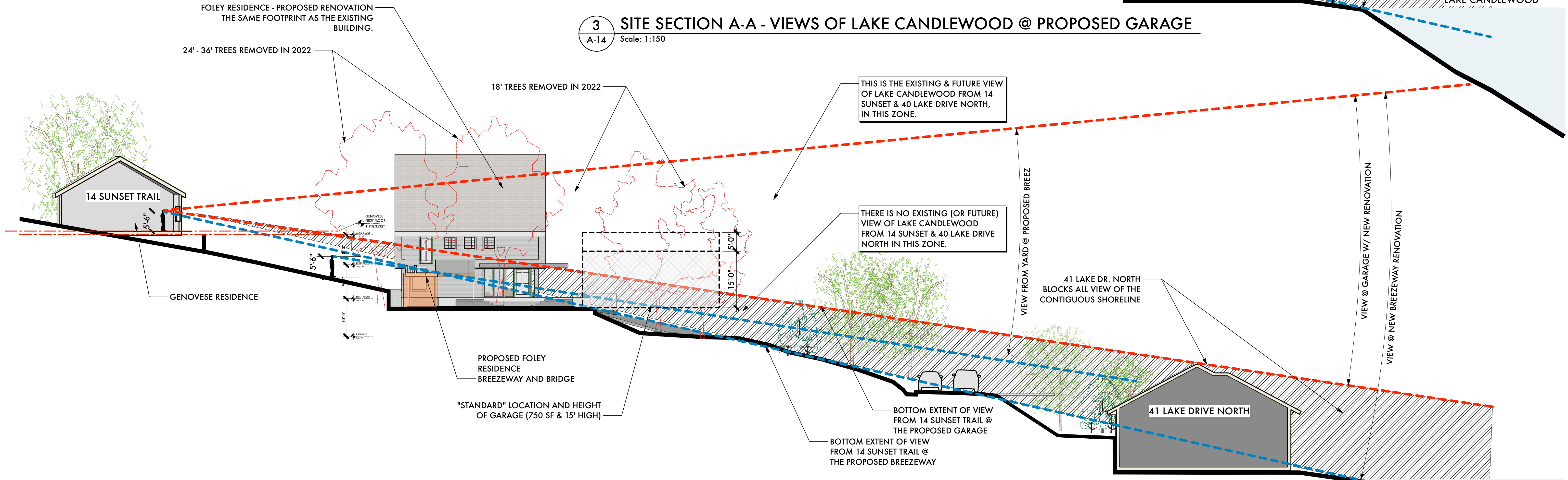
2 SITE SECTION B-B VIEW OF LAKE CANDLEWOOD AT PROPOSED BREEZEWAY A-14 Scale: 1:150
