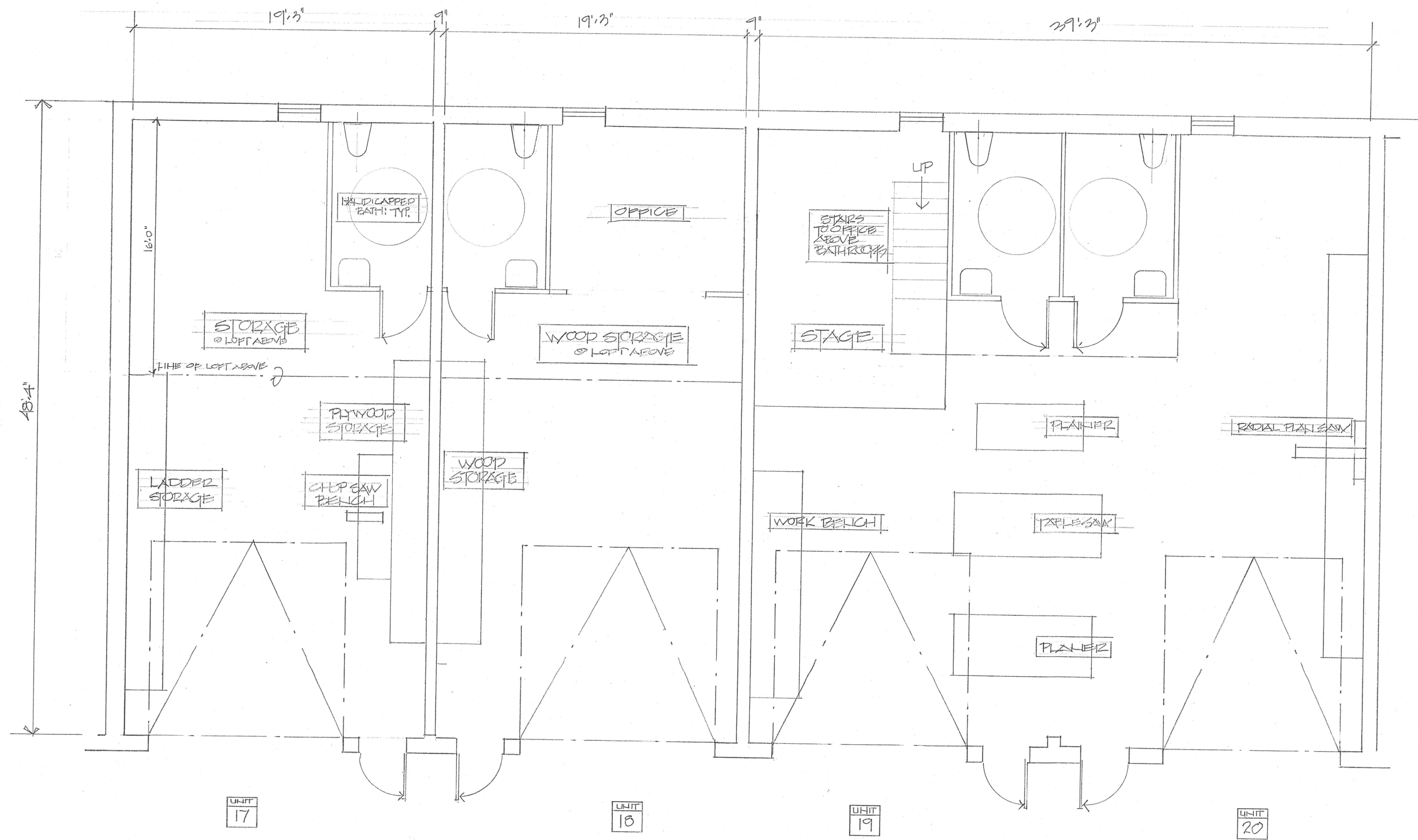
1 FLOORPLAN: UNITS 17-20
